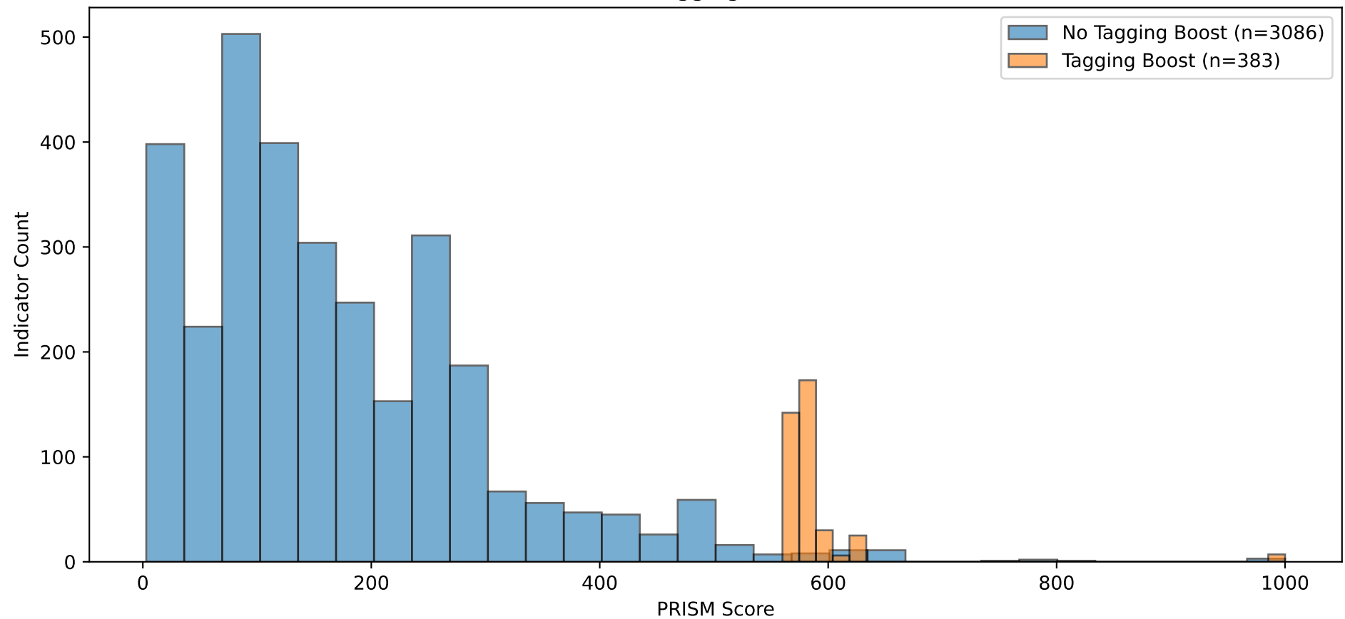
Score Distribution: Tagging Boost vs Non-Boosted
